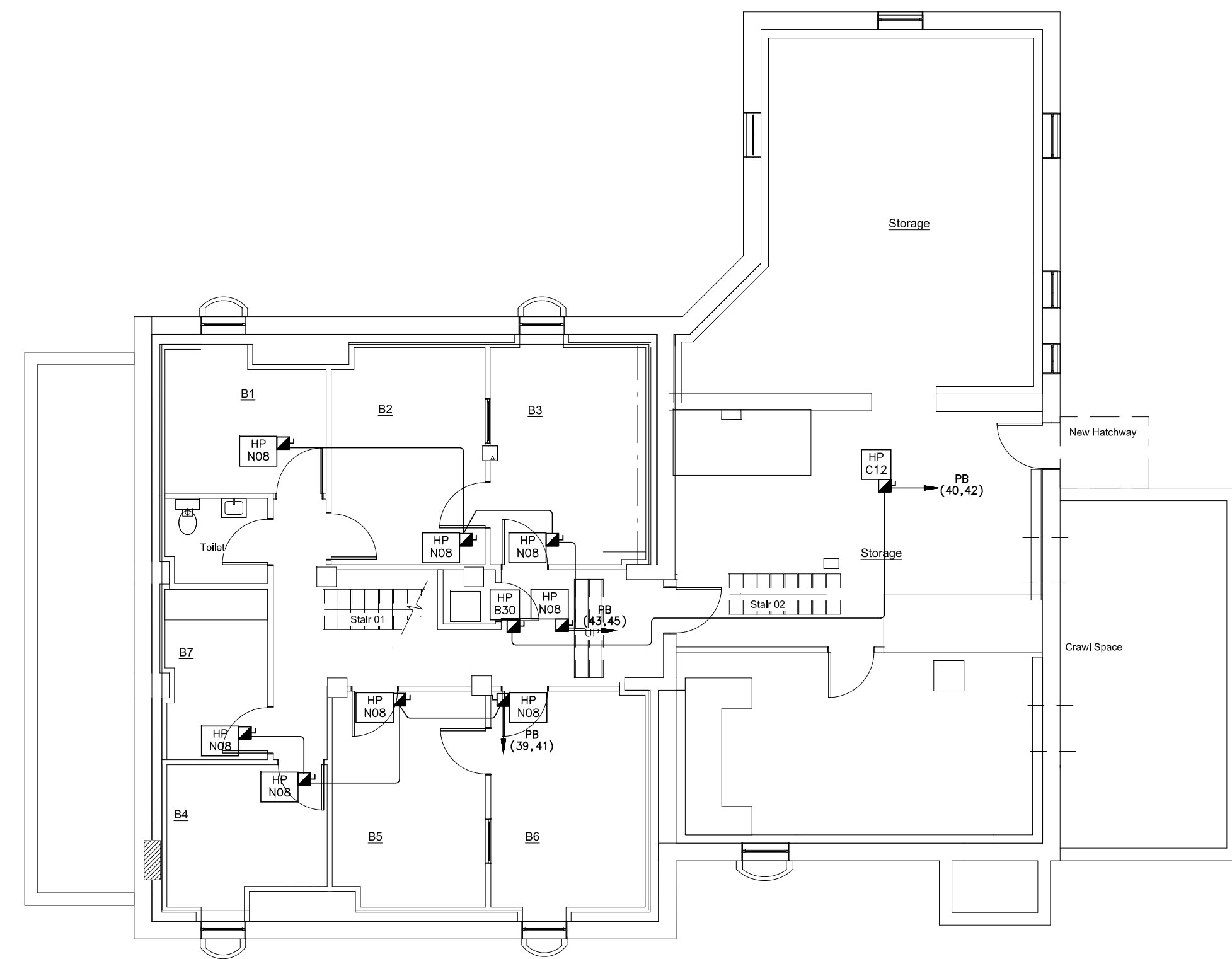
BASEMENT FLOOR PLAN - HVAC ELECTRICAL Scale: 1/8"=1'-0"
