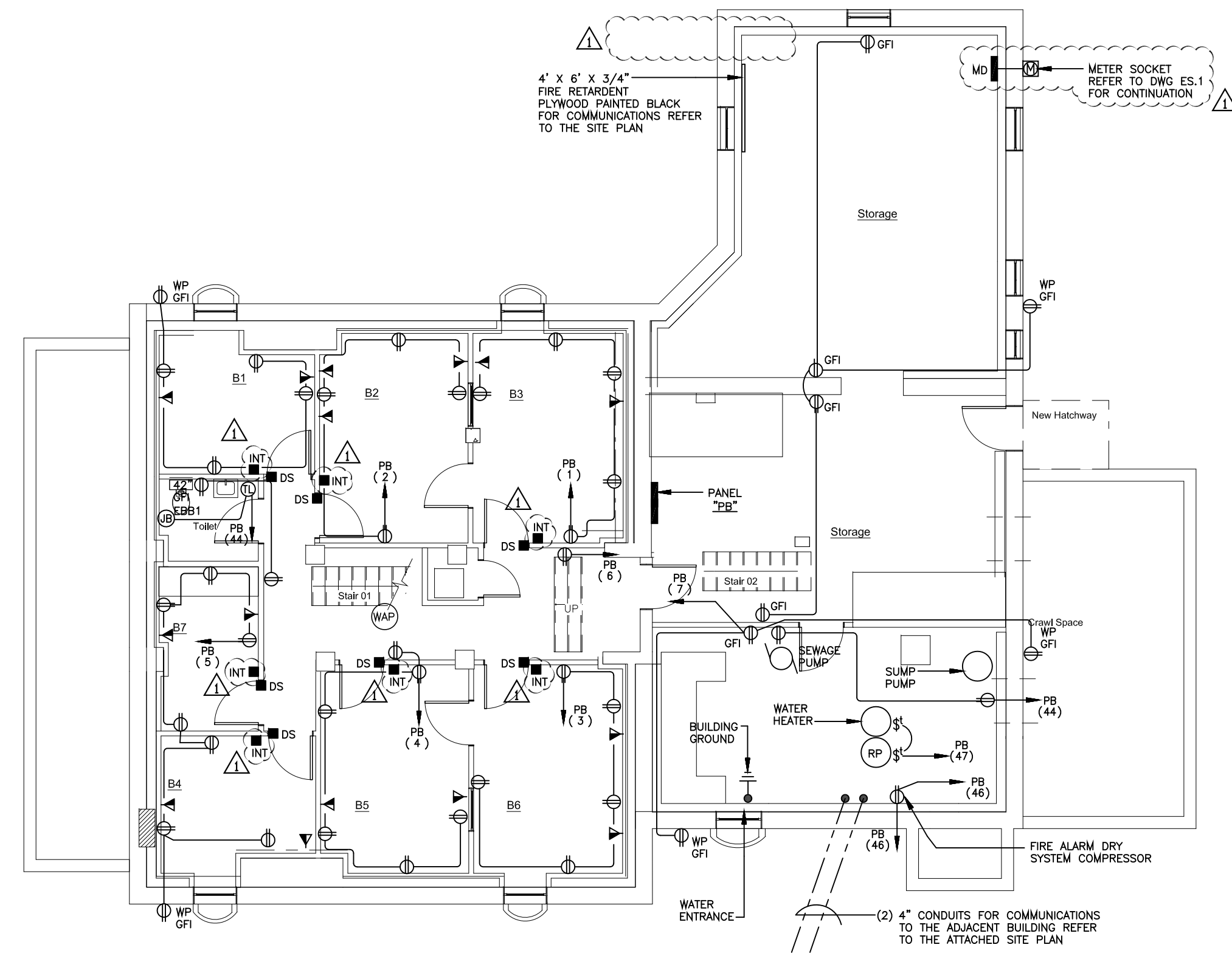
BASEMENT FLOOR PLAN - POWER Scale: 1/8"=1'-0"
