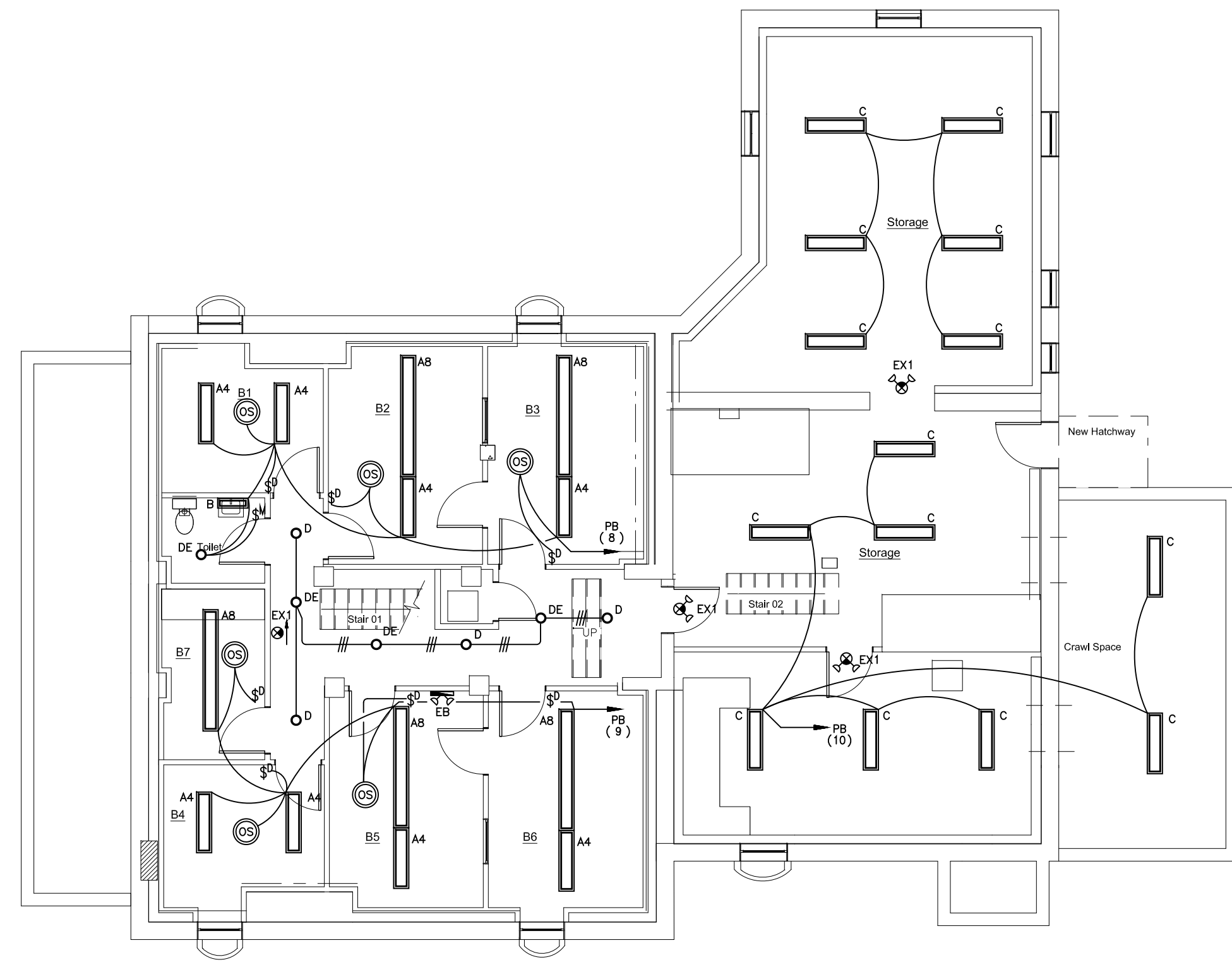
BASEMENT FLOOR PLAN - LIGHTING Scale: 1/8"=1'-0"
